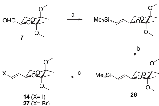
Scheme 5. Alternative synthetic route to obtain E -vinyl halides 14 and 27 . Reagents and conditions: (a) \text{CpTi}(\text{CH}_2\text{SiMe}_3)_3 , 1,4-dioxane, reflux, overnight, 38%; (b) AIBN (cat.), \text{PhSH} (cat.), toluene, 80^\circ\text{C} , 5 h, 91%; (c) NIS or NBS, \text{CH}_3\text{CN} , darkness, 85-90^\circ\text{C} , 1 h, 50% (iodide), 34% (bromide).
