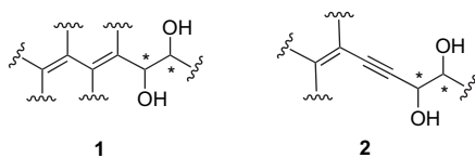
Scheme 1. Common motifs found in many biologically active compounds.
