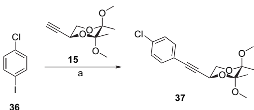
Scheme 10. Chemoselective Sonogashira reaction of 36 with 15 . Reagents and conditions: (a) 5 mol % Pd(PPh 3 ) 2 Cl 2 , 5 mol % CuI, Hünig's base (DIPEA), toluene, 24 h.
