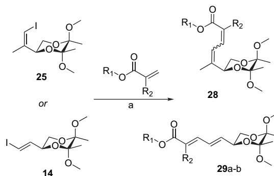
Scheme 6. Heck reactions. Reagents and conditions: (a) 10 mol % \text{Pd}_2(\text{dba})_3 , 20 mol % \text{P}(t\text{-Bu})_3 , \text{Cy}_2\text{MeN} (1.5 equiv), toluene, 80-120^\circ\text{C} , 24 h.
