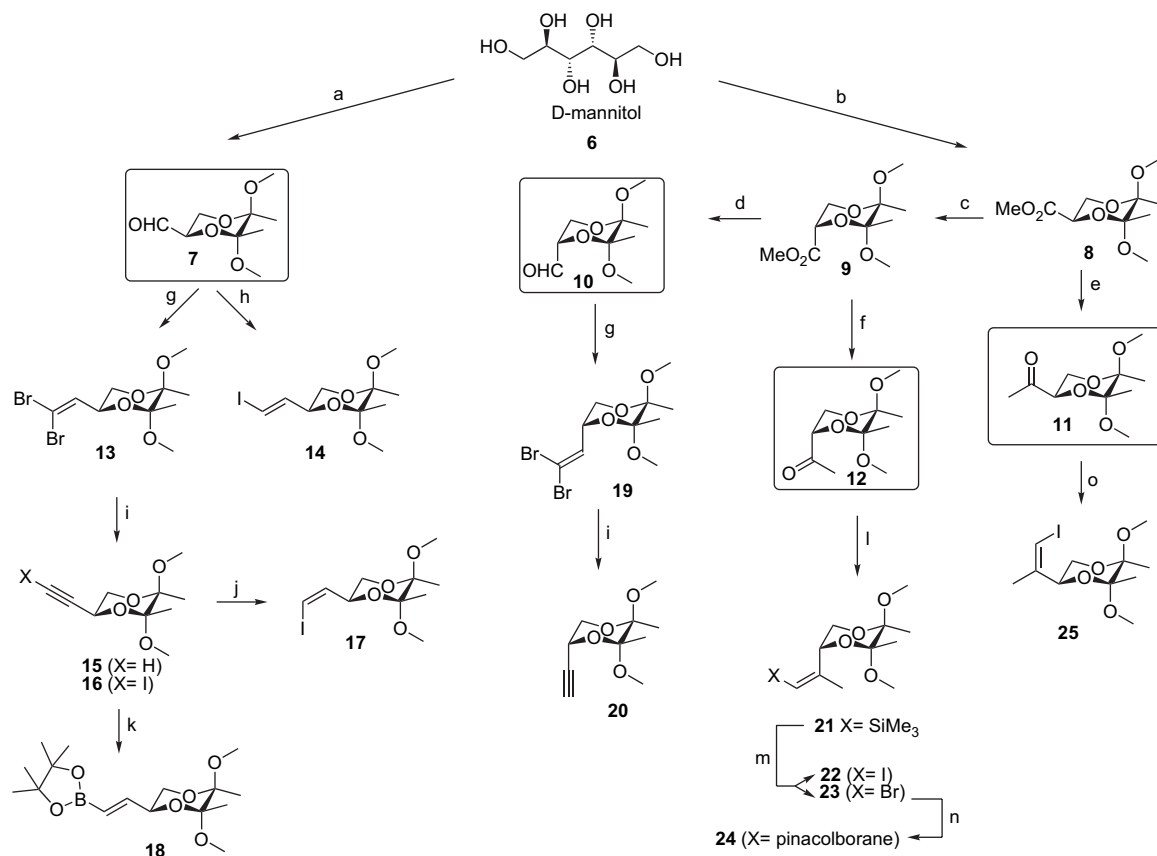
Scheme 4. Synthetic route to monosubstituted BDA-protected asymmetric diols containing vinyl halides, vinyl boronates and alkynyl functionalities. Reagents and conditions: (a) butanedione, \text{HC}(\text{OMe})_3 , \text{BF}_3 \cdot \text{Et}_2\text{O} (cat.), MeOH, rt, 5 h; then \text{NaIO}_4 , \text{CH}_2\text{Cl}_2 , rt, 16 h, 40%; (b) butanedione, \text{HC}(\text{OMe})_3 , \text{BF}_3 \cdot \text{Et}_2\text{O} (cat.), MeOH, rt, 5 h; then \text{NaIO}_4 , \text{MeOH}-\text{H}_2\text{O} , rt, 16 h; then \text{Br}_2 , \text{NaHCO}_3 , rt, 30 min, 46%; (c) LDA, THF, -78^\circ\text{C} , 30 min; then t\text{-BuOH} , -78^\circ\text{C} , 30 min, 48%; (d) \text{LiAlH}_4 , THF; then (\text{COCl})_2 , DMSO, \text{Et}_3\text{N} , \text{CH}_2\text{Cl}_2 , 83%; (e) \text{Cp}_2\text{TiMe}_2 , toluene, 65^\circ\text{C} , overnight; then \text{NH}_4^+\text{Cl}^- (aq), 60^\circ\text{C} , 6 h, 70–80% over 2 steps; (f) \text{MeLi} \cdot \text{LiBr} , \text{CH}_2\text{Cl}_2 , -78^\circ\text{C} , 2 h, 50–71%; (g) \text{CBr}_4 , \text{PPh}_3 , \text{Zn} , \text{CH}_2\text{Cl}_2 , rt, 2 h, 94–96%; (h) \text{CrCl}_2 , \text{CHI}_3 , THF, rt, 24 h, 45%; (i) n\text{-BuLi} , THF, -78^\circ\text{C} to rt; then \text{NH}_4\text{Cl} (aq) or \text{I}_2 , 79–100%; (j) \text{KO}_2\text{C}\equiv\text{NCO}_2\text{K} , MeOH, AcOH, rt, 30% over 2 steps; (k) pinacolborane, 80^\circ\text{C} , 6 h, 70%; (l) \text{CpTi}(\text{CH}_2\text{SiMe}_3)_3 , 1,4-dioxane, reflux, 24 h, 63%; (m) NIS or NBS, \text{CH}_3\text{CN} , darkness, rt, 16 h, 97% (iodide), 1 h, 100% (bromide); (n) pinacolborane dimer, \text{PdCl}_2(\text{PPh}_3)_2 (cat.), \text{KOPh} , toluene, 80^\circ\text{C} , 90 min, 28%; (o) \text{ICH}_2\text{PPh}_3\text{I} , \text{NaHMDs} , THF, -78^\circ\text{C} to rt, 3 h 30 min, 15–36%.
