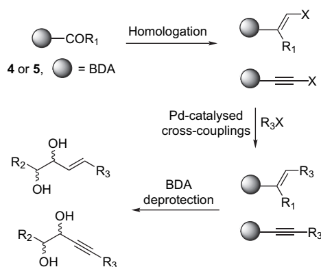
Scheme 3. General strategy to obtain motifs 1 and 2 .
