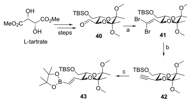
Scheme 12. Applying the methodology in bisubstituted BDA-protected asymmetric diols. Reagents and conditions: (a) CBr 4 , PPh 3 , Zn, CH 2 Cl 2 , rt, 2 h, 84%; (b) n -BuLi, THF, −78 °C to rt; then NH 4 Cl (satd), 100%; (c) pinacolborane, 100 °C, 24 h, 100%.
