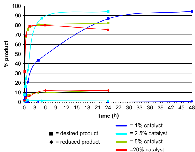
Figure 1. Kinetic study of the Suzuki reaction between 14 and trimethylboroxine using different catalyst loading.
