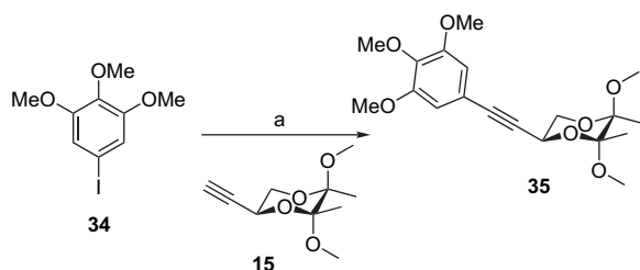
Scheme 9. Sonogashira reaction of 34 with BDA-protected alkyne 15 . Reagents and conditions: Pd(PPh 3 ) 2 Cl 2 , CuI, Hünig's base (1.5 equiv), toluene.
