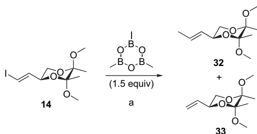
Scheme 8. Suzuki reaction with trimethylboroxine. Reagents and conditions: (a) PdCl 2 (dppf)·CH 2 Cl 2 , K 2 CO 3 (3 equiv), 1,4-dioxane, 110 °C.
