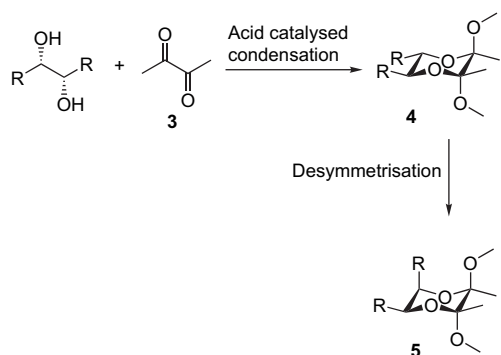
Scheme 2. Butanediactal (BDA)-protected diols containing carbonyl functionalities. R=CO 2 Me.
