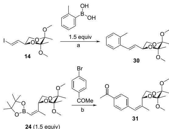
Scheme 7. Suzuki reactions. Reagents and conditions: (a) 5 mol % Pd(OAc) 2 , 7.5 mol % SPhos, K 3 PO 4 (2 equiv), toluene, 110 °C, 70%; (b) 20 mol % Pd(OAc) 2 , 20 mol % SPhos, K 3 PO 4 , THF, rt, 24 h, 65%.
